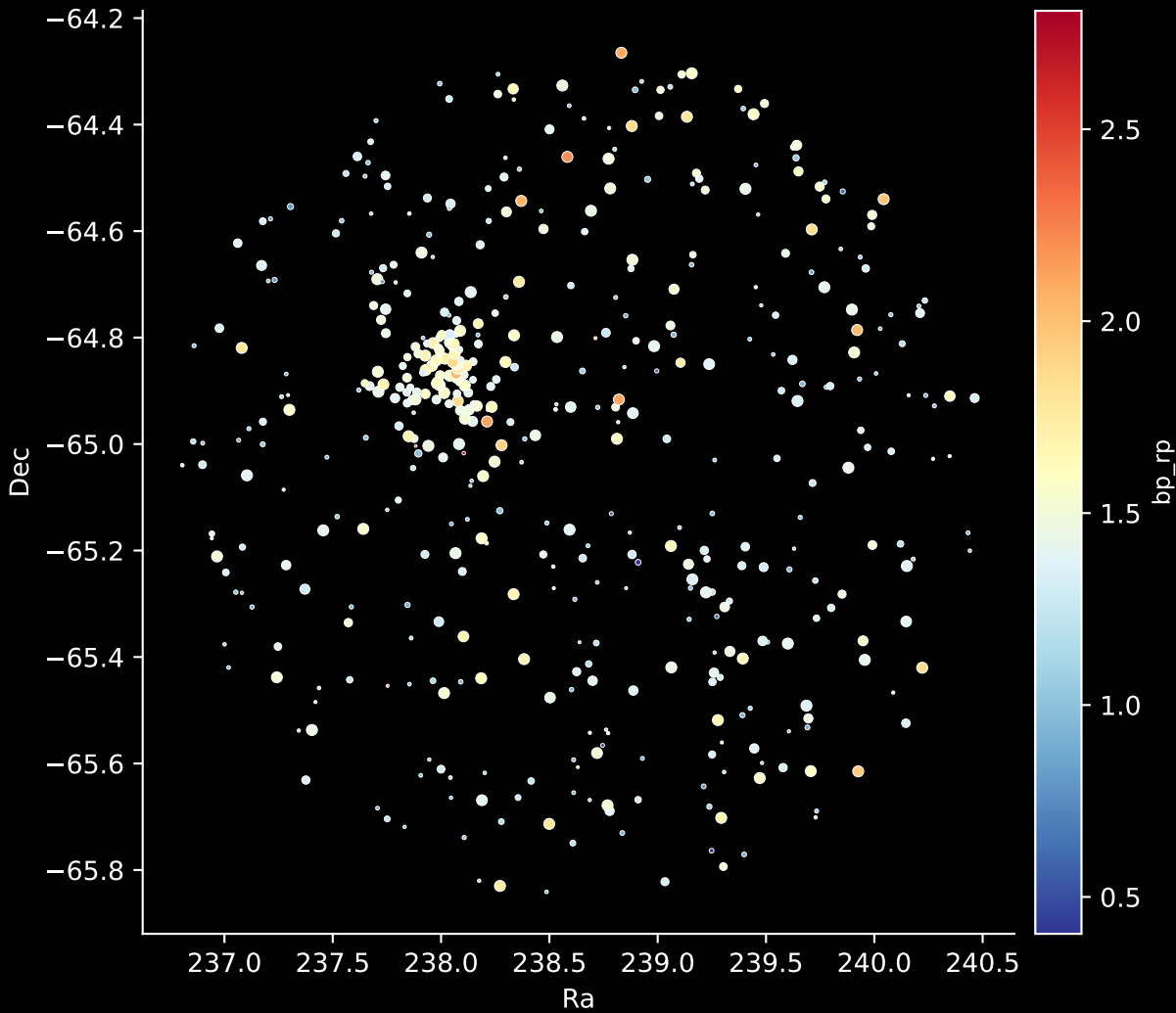
APOGEE DR17 Field: [N2808] Stars: 476
