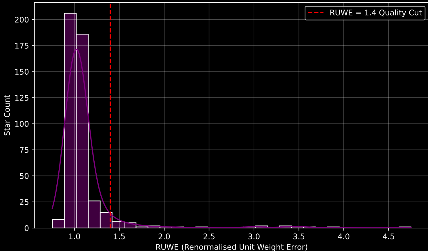
GAPOGEE DR17 Field [N2808] RUWE Distribution (n= 467)
