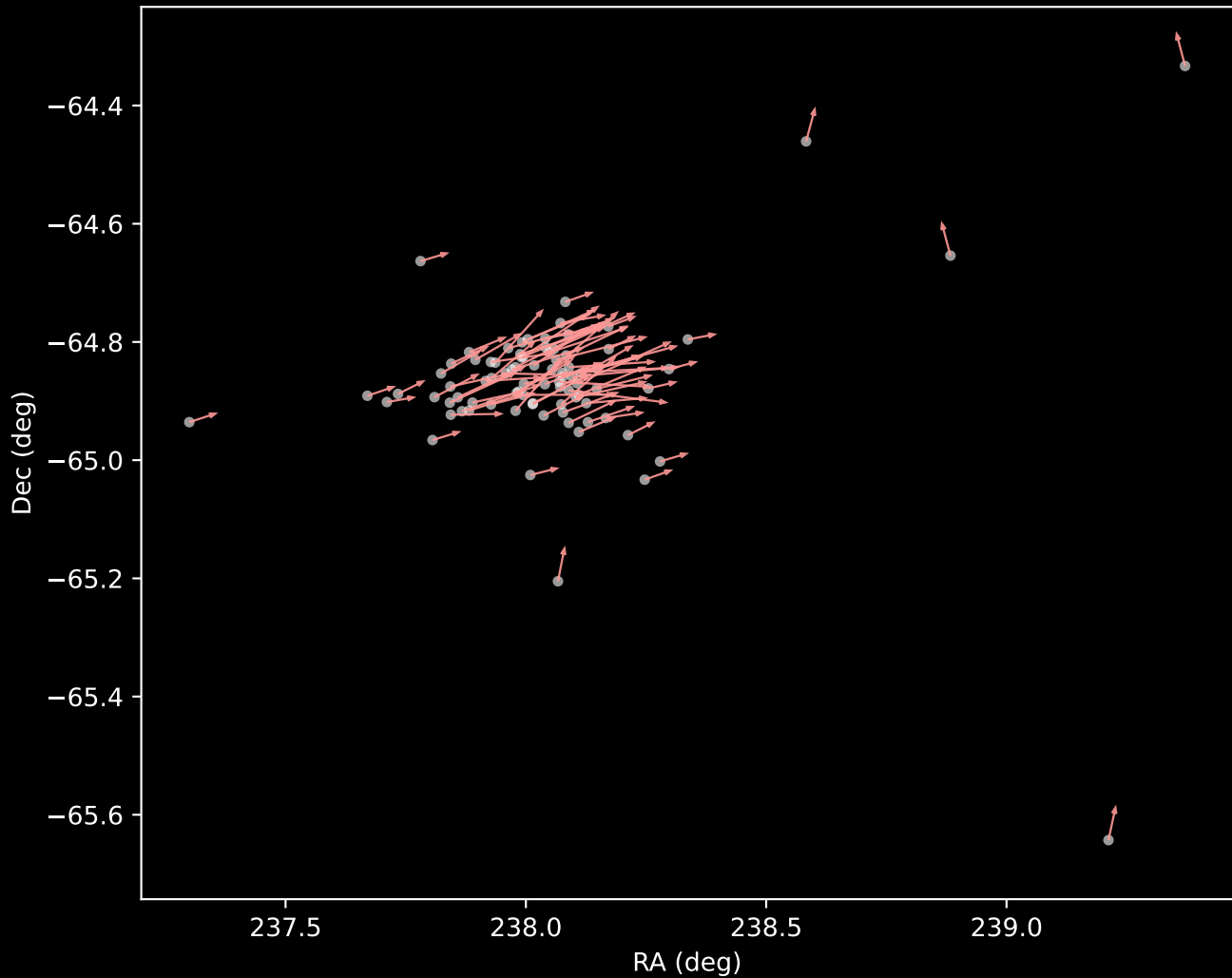
APOGEE DR17 Cluster 7 Proper Motion Vectors (n=86)
