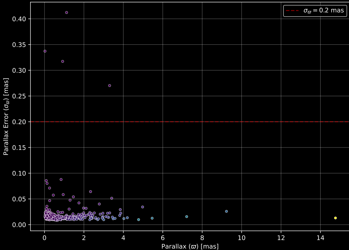
APOGEE DR17 Field: [N2808] Parallax Quality (n= 476)
