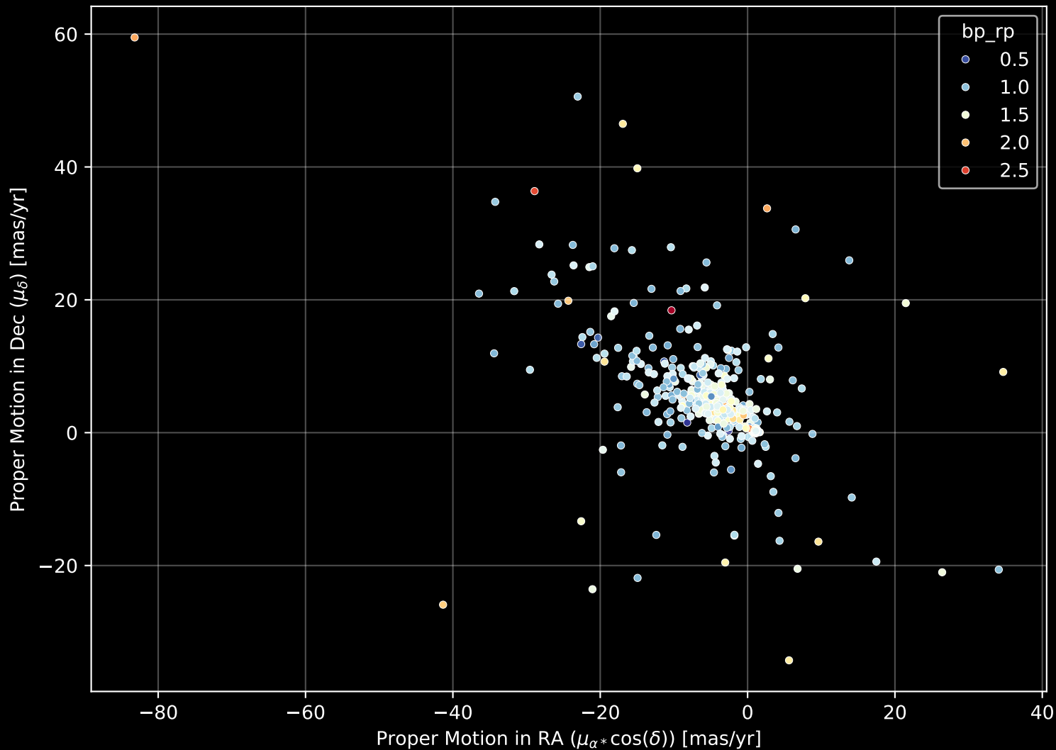
APOGEE DR17 Field: [N2808] Proper Motion Diagram (n= 476)
