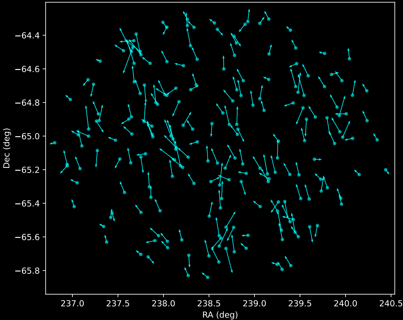
APOGEE DR17 Noise Stream Proper Motion Vectors (n=203)
