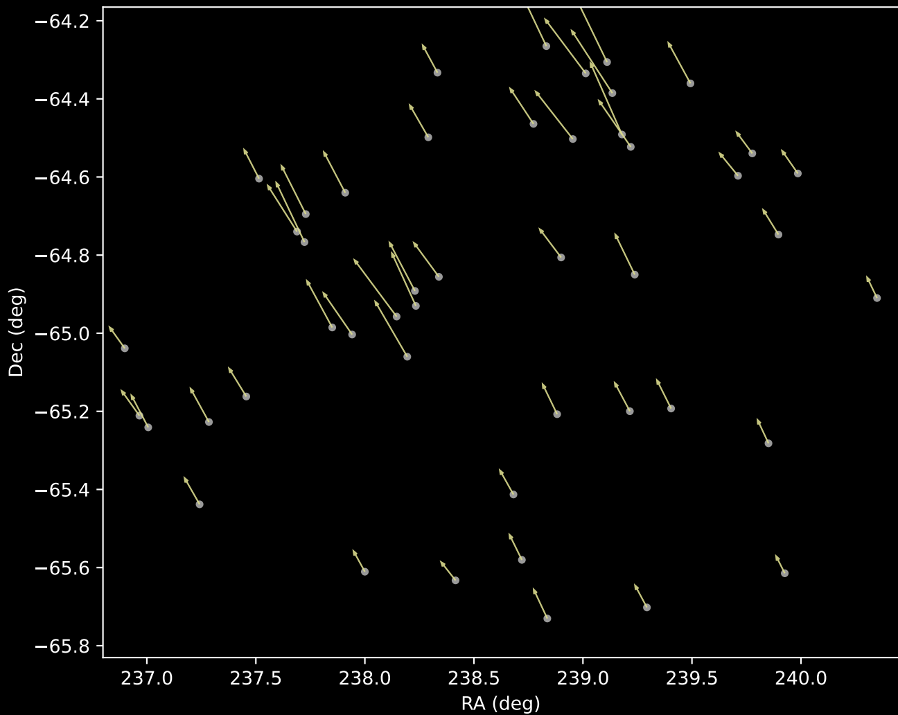
APOGEE DR17 Cluster 17 Proper Motion Vectors (n=47)
