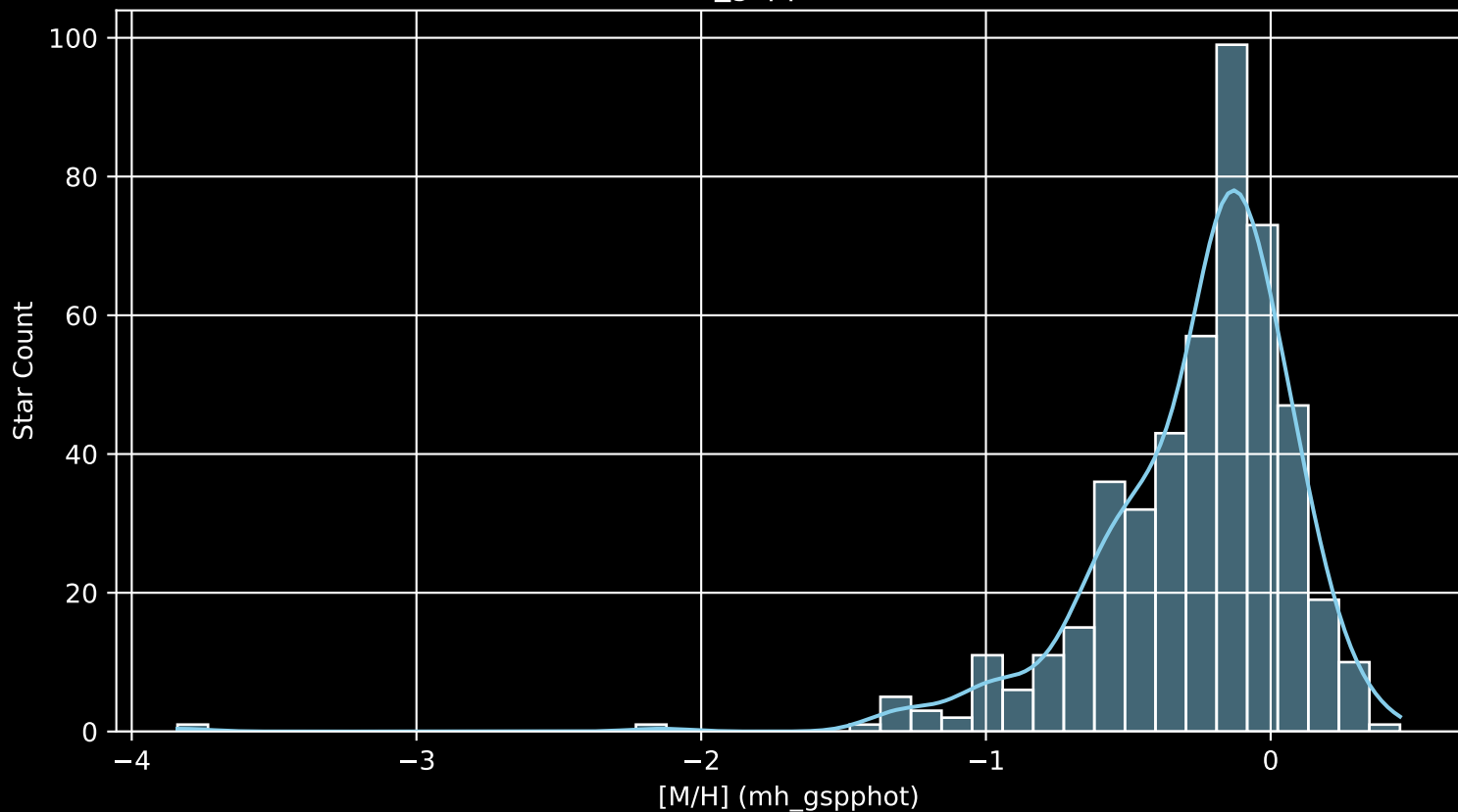
APOGEE DR17 Field: [N2808 [M/H] (mh_gspphot) (n= 473)
