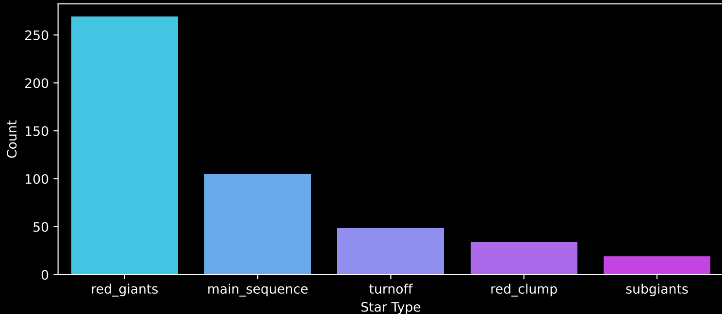
APOGEE DR17 Field: [N2808] Count plot of Star Type
