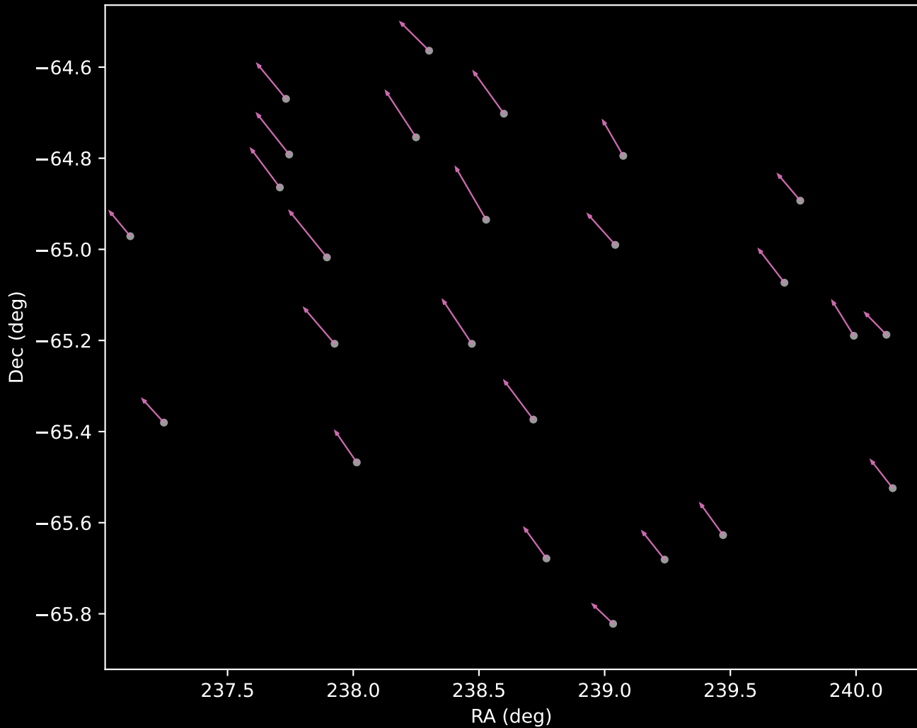
APOGEE DR17 Cluster 12 Proper Motion Vectors (n=25)
